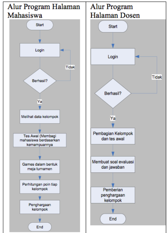
Gambar 3 Alur Program
