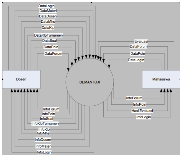
Gambar 5 DFD Level 0
